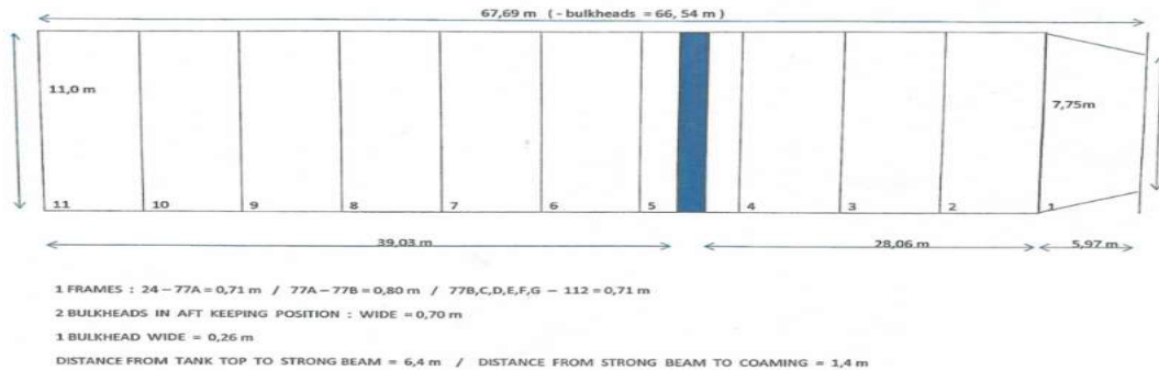
MV "VALENTINA" HOLD DIMENSIONS
